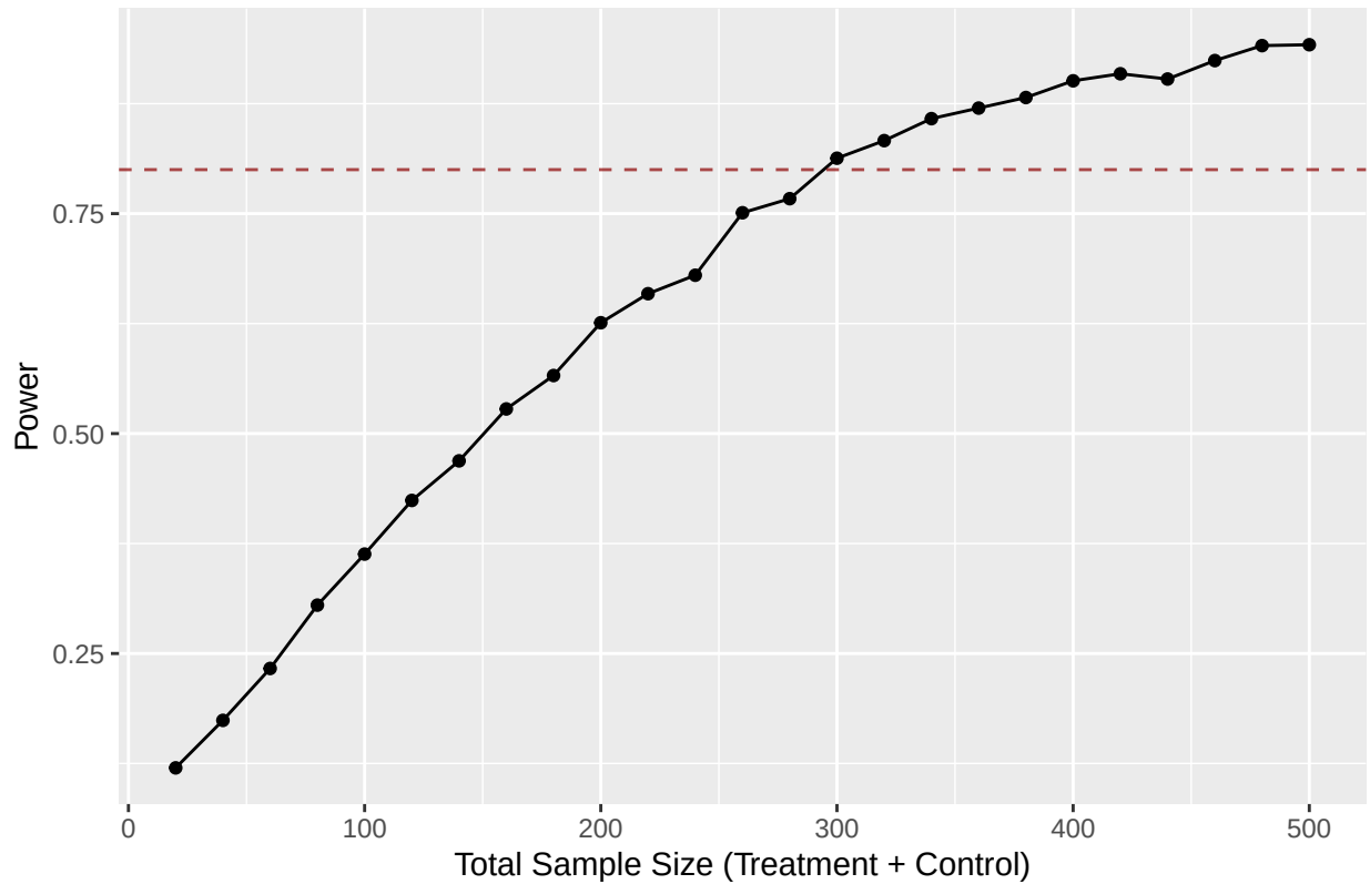
Power vs. Sample Size [Effect Size = 15, SD = 45]
