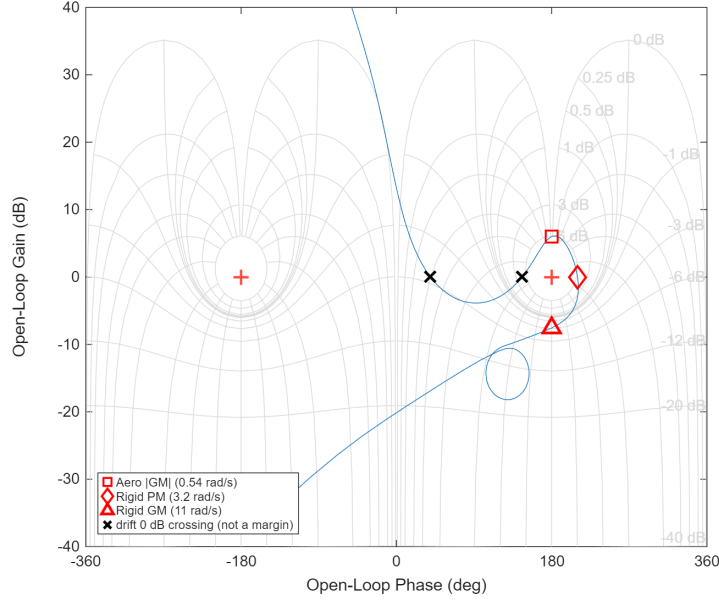
Figure 11: Task 2 — retained full-loop Nichols (deep notch, re-tuned PD) in the launch-vehicle convention (critical point +180^\circ ): aerodynamic gain margin ( |GM_a| = 6 dB), rigid phase margin ( 30^\circ ) and the high-frequency rigid gain margin (set by the actuator lag) are marked. The bending mode is gain-stabilised, so its lobe stays well below 0 dB near \omega_{BM} rather than threading the critical point.
