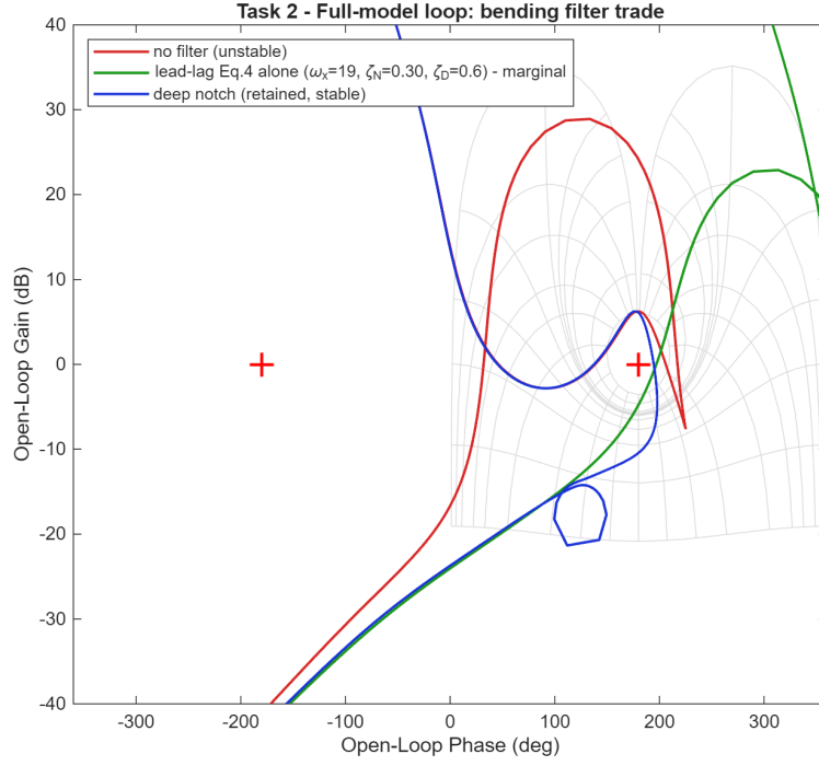
Figure 12: Task 2 — bending-filter trade on the Nichols chart (launch-vehicle convention, critical point +180^\circ ; a common phase shift aligns the three loops at the rigid crossover): without a filter the +29 dB bending lobe (red) wraps over the critical point and the loop is unstable; the best Eq.-4 lead-lag alone (green) rotates the lobe but only marginally; the deep notch (blue) pushes the bending lobe far below 0 dB (the small loop near -18 dB), gain-stabilising it.
