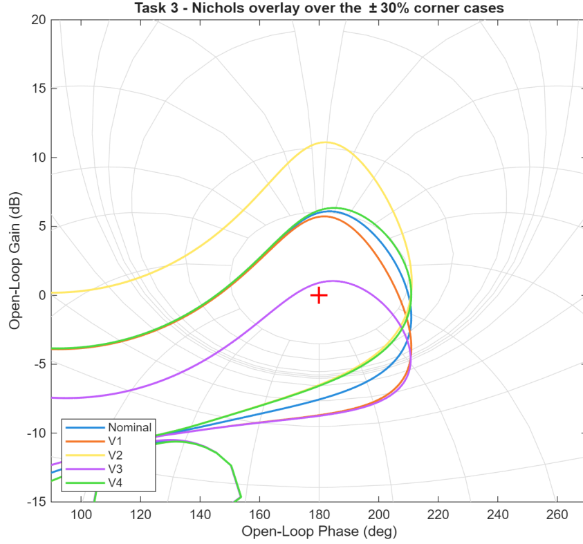
Figure 17: Task 3 — Nichols overlay over the nominal case and the four uncertainty-box vertices (launch-vehicle convention, critical point +180^\circ ). Every corner stays clear of the critical point; V3 (max instability, min authority) rides closest, its aerodynamic gain margin nearly vanishing.
