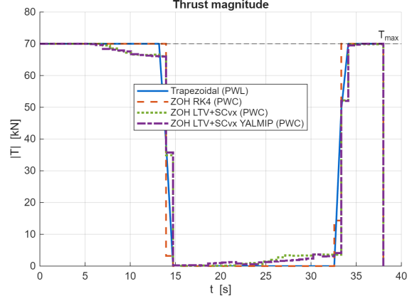
(b) Thrust magnitude: PWL (trapezoidal) vs PWC (ZOH).
