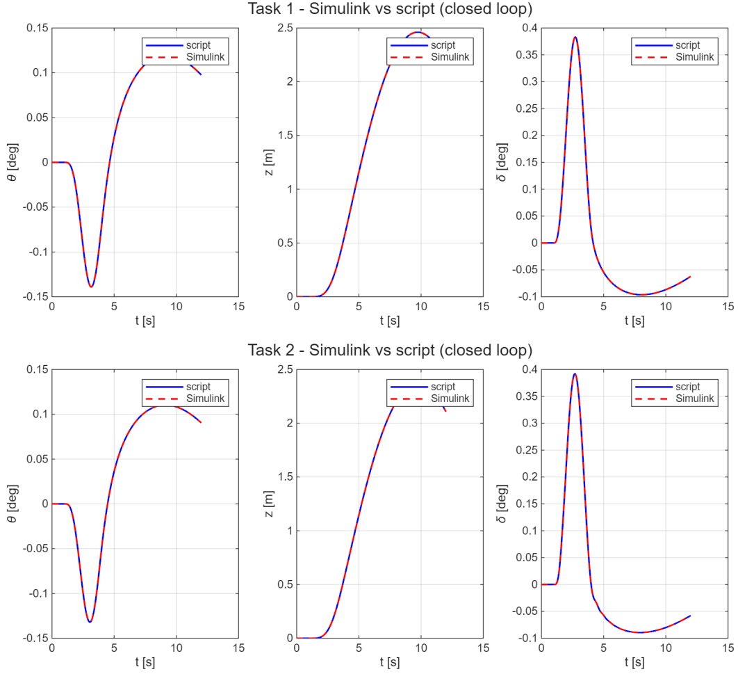
Figure 12: Simulink (dashed) versus script (solid) closed-loop response to the sizing 1-cosine gust: pitch \theta , lateral drift z and TVC deflection \delta . Top: Task 1 (rigid plant, ideal actuator); bottom: Task 2 (flexible plant, TVC servo, Padé delay and bending notch). The traces are indistinguishable at plot scale.
