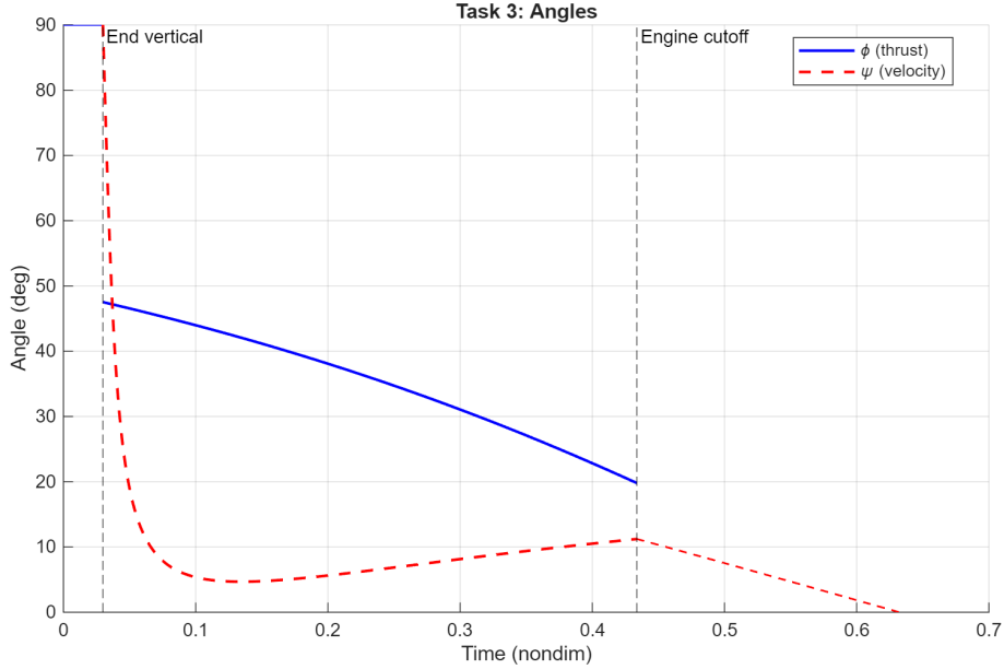
Figure 6: Task 3: thrust angle \phi and velocity angle \psi across all three phases. Vertical dashed lines mark phase transitions.
