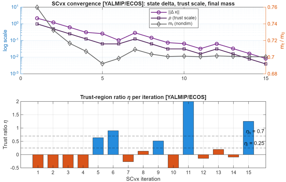
Figure 8: SCvx convergence, variant (c) (YALMIP+ECOS inner solver). Panels as in Fig. 7.
