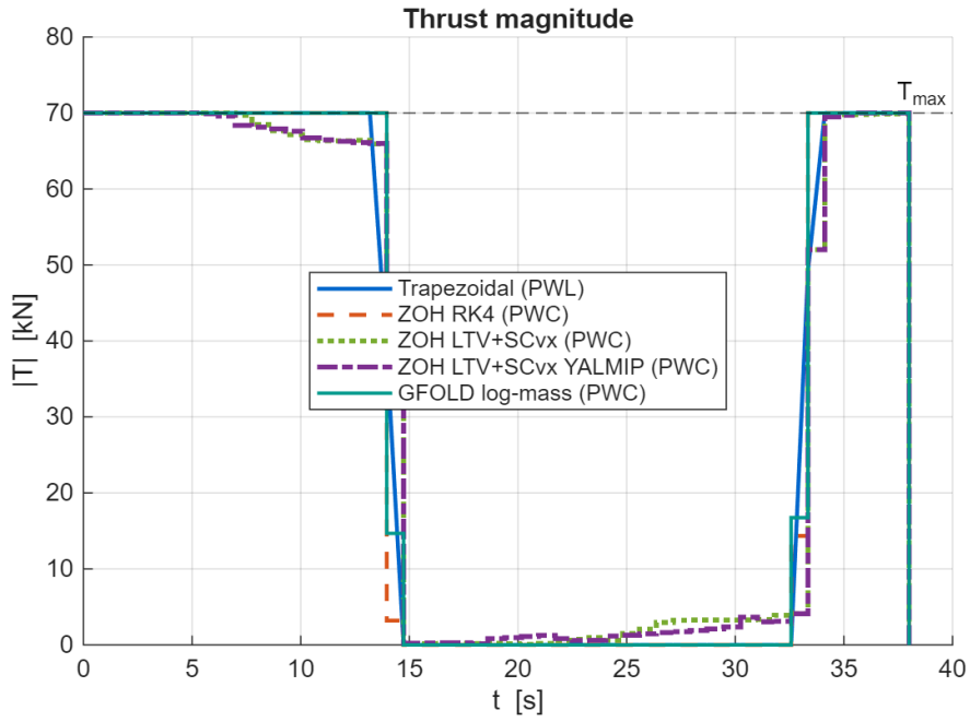
Figure 5: Comparison of the five transcriptions at t_f = 38 s.
