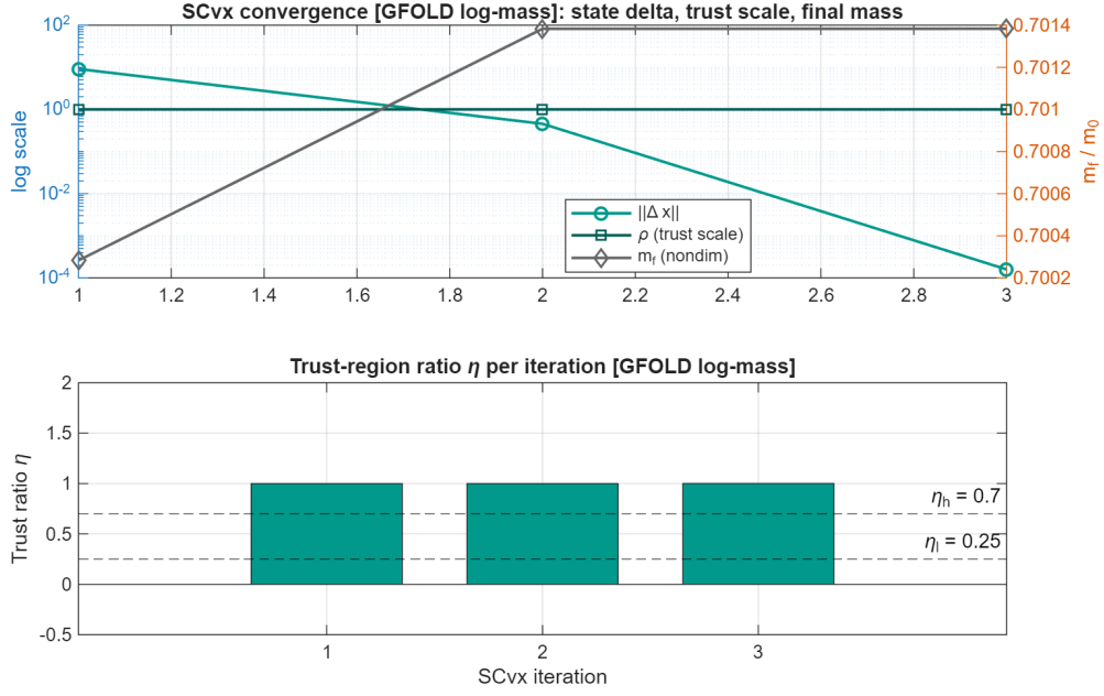
Figure 9: SCvx convergence, variant (d) (GFOLD log-mass): self-started from the analytic max-thrust mass profile, every step accepted with \eta \approx 1 , converged in three iterations. Panels as in Fig. 7.
