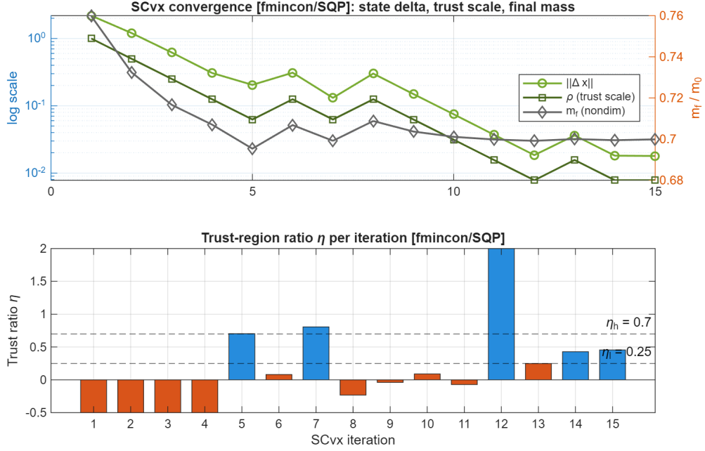
Figure 7: SCvx convergence, variant (b) (fmincon/SQP inner solver). Top panel: iterate change \|\mathbf{x}^{(j+1)} - \mathbf{x}^{(j)}\|_2 (left axis, log), trust scale \rho , and final mass m_f (right axis) per outer iteration. Bottom panel: trust-region ratio \eta against the acceptance band [\eta_l, \eta_h] = [0.25, 0.7] , with rejected steps highlighted in orange.
