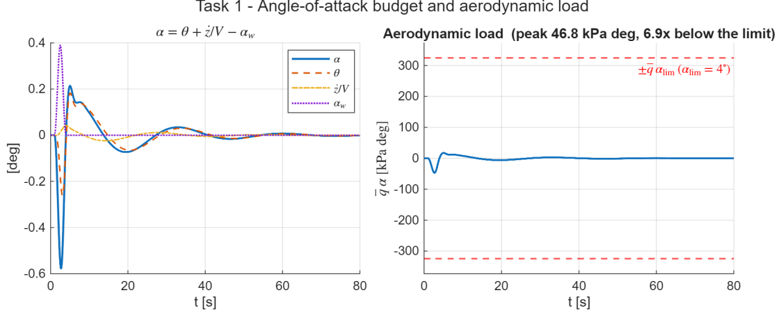
Figure 9: Task 1 — angle-of-attack budget \alpha = \theta + \dot{z}/V - \alpha_w (left) and aerodynamic load indicator \bar{q} \alpha (right) during the severe gust. The attitude loop pitches into the relative wind, so \theta and -\alpha_w add: the peak incidence ( 0.577^\circ ) exceeds the gust alone ( 0.39^\circ ). The trace is kept signed , as customary for planar time histories (the sign carries the loading direction and shows the control and wind contributions adding); the structural check is on the modulus, against the symmetric allowable \pm \bar{q} \alpha_{\text{lim}} (dashed, \alpha_{\text{lim}} = 4^\circ representative of a slender launcher), which the response clears by a factor 6.9.
