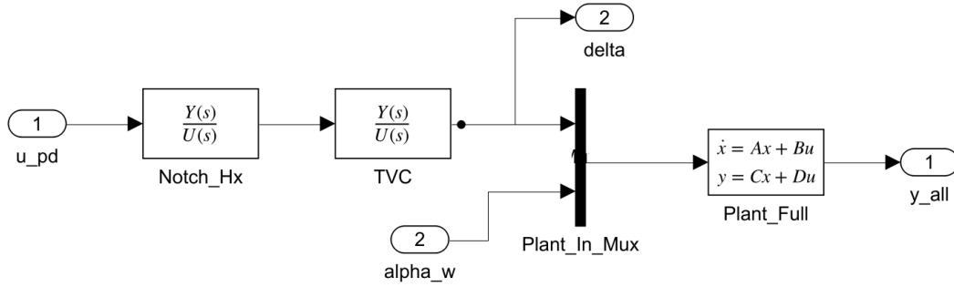
(b) Full.TVC_Notch (Tasks 2-3): notch, TVC servo with Padé delay, flexible plant.
