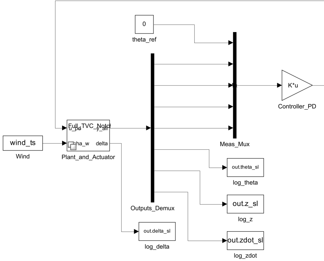
Figure 20: Root of the Simulink mirror: the PD controller ( Controller_PD ), the variant plant and actuator block ( Plant_and_Actuator ), the wind input ( wind_ts ) and the signal logging. The measurement bus feeds the controller, whose output u_{pd} drives the plant; the demultiplexed states close the loop and are logged.
