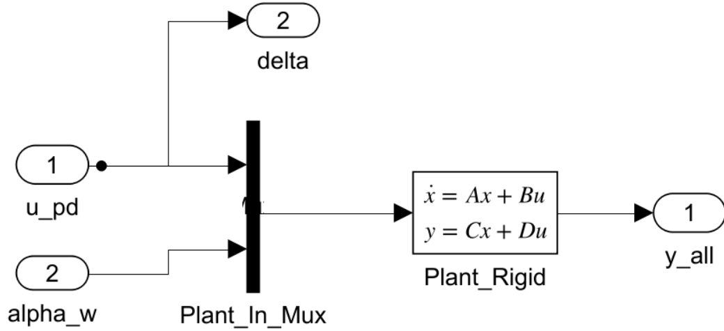
(a) Rigid_Ideal (Task 1): rigid plant, ideal actuator ( \delta = u_{pd} ).
