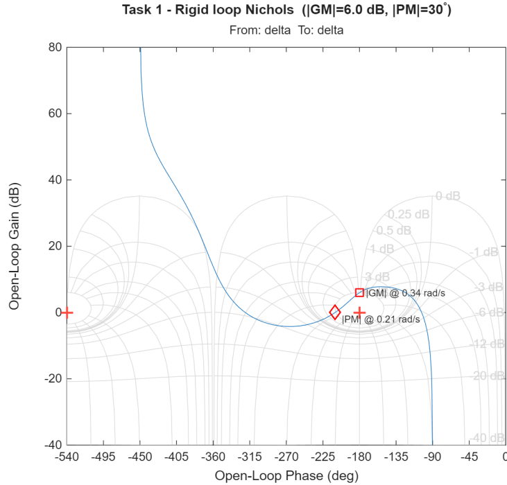
Figure 6: Task 1 — Nichols chart of the rigid open-loop transfer. The loop is conditionally stable; the design meets |GM| \approx 6 dB and |PM| \approx 30^\circ (markers at the crossover frequencies).
