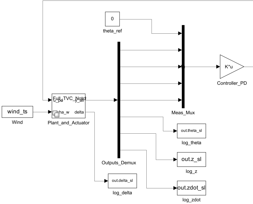
Figure 18: Root of the Simulink mirror: the PD controller ( Controller_PD ), the variant plant and actuator block ( Plant_and_Actuator ), the wind input ( wind_ts ) and the signal logging. The measurement bus feeds the controller, whose output u_{pd} drives the plant; the demultiplexed states close the loop and are logged.
