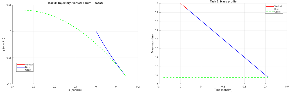
(a) Trajectory: vertical climb (red), burn (blue), coast (green dashed).
