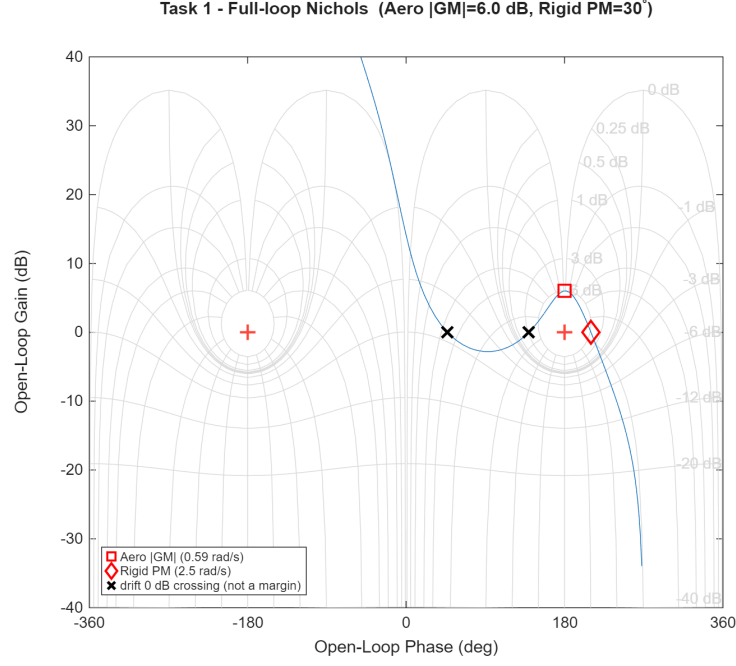
Figure 6: Task 1 — full-loop Nichols in the launch-vehicle convention (critical point at +180^\circ ). The loop comes from the top (lateral-drift integrator); the design meets |GM_a| \approx 6 dB (aerodynamic, at +180^\circ ) and PM \approx 30^\circ (rigid-body, at the 2.45 rad/s crossover).
