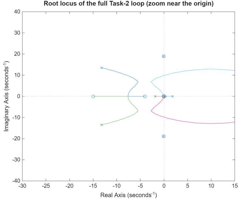
Figure 12: Task 2 — root locus of the full loop (flexible plant, TVC servo, Padé delay and notch), zoomed near the origin ( \times : open-loop poles; \circ : open-loop zeros). The bending poles sit near \omega_{BM} \approx 18.9 rad/s and the design is stable (all closed-loop poles in the left half-plane); the delay’s right-half-plane zeros lie far outside this window.
