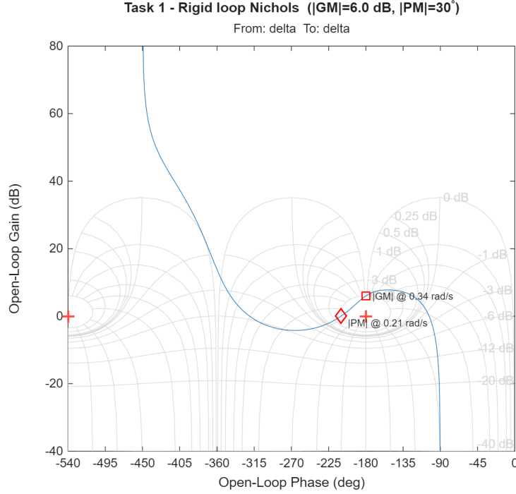
Figure 1: Task 1 — Nichols chart of the rigid open-loop transfer. The loop is conditionally stable; the design meets |GM| \approx 6 \text{ dB} and |PM| \approx 30^\circ (markers at the crossover frequencies).
