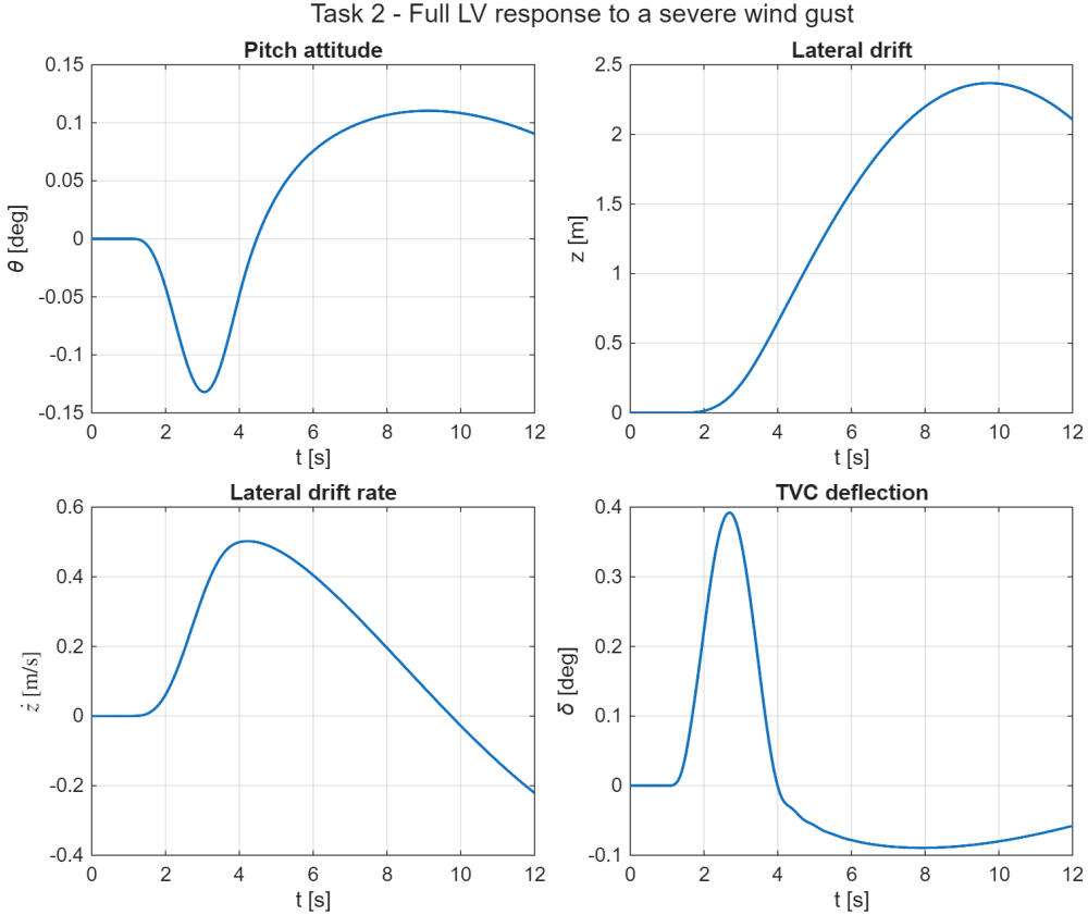
Figure 5: Task 2 — full-model response to the severe wind gust: pitch attitude \theta , lateral drift z , drift rate \dot{z} and TVC deflection \delta .
