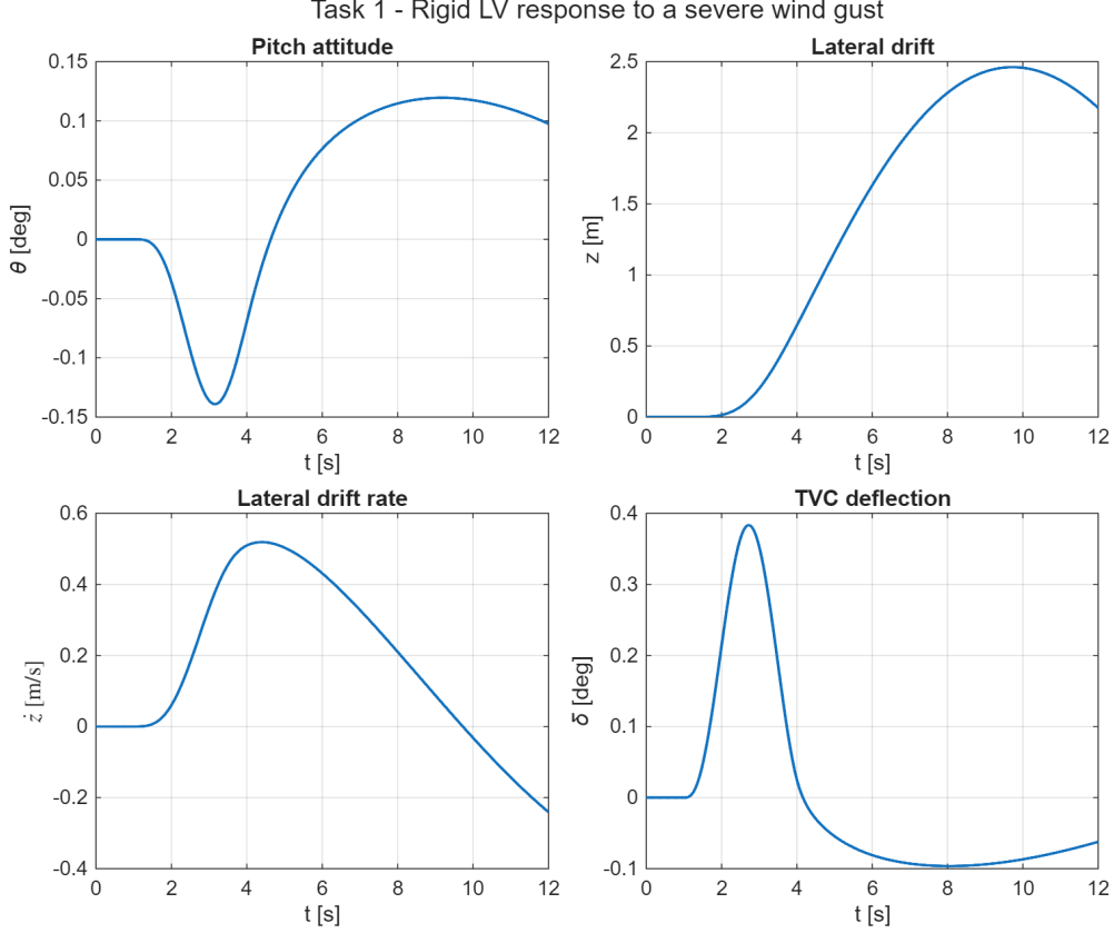
Figure 2: Task 1 — response to a severe wind gust: pitch attitude \theta , lateral drift z , drift rate \dot{z} and TVC deflection \delta .
