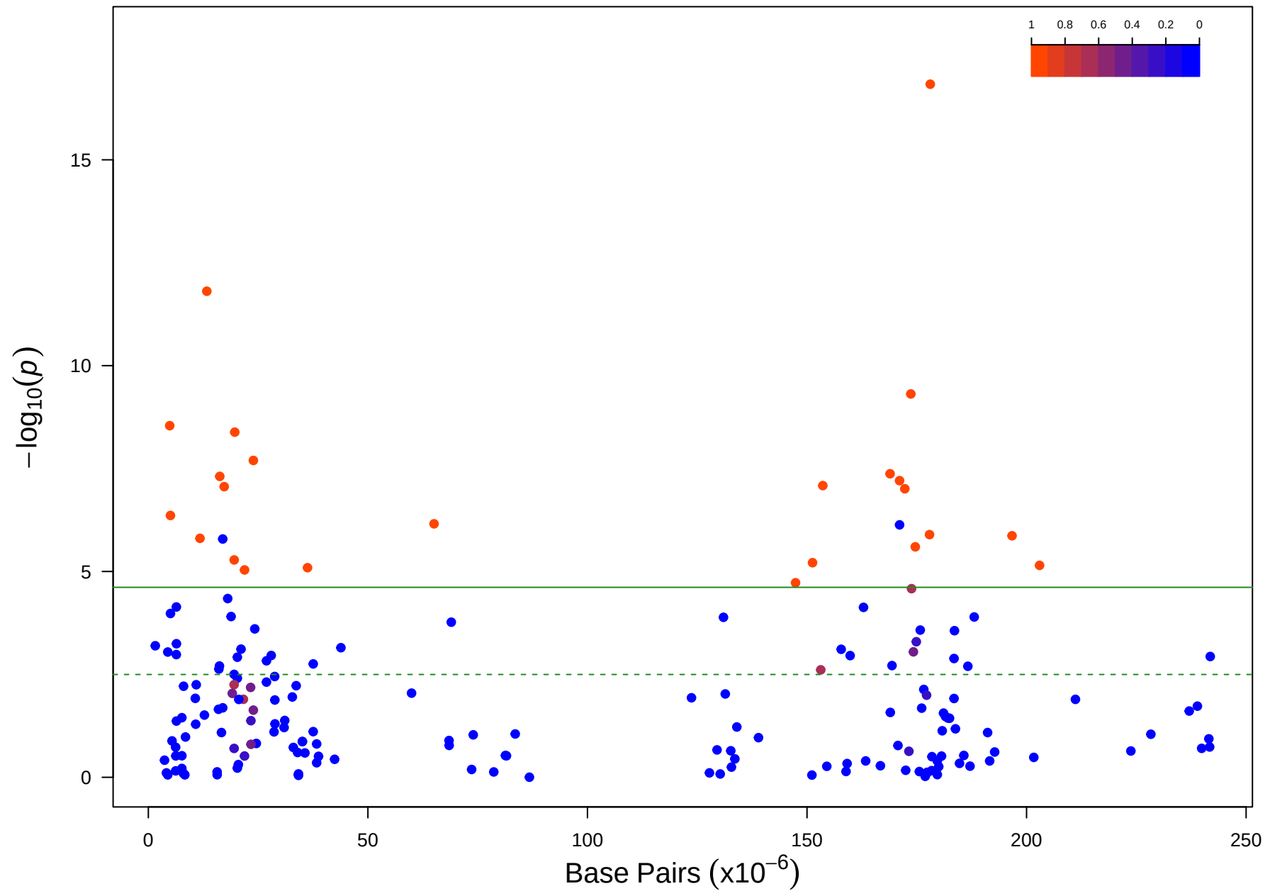
Chromosome 4
