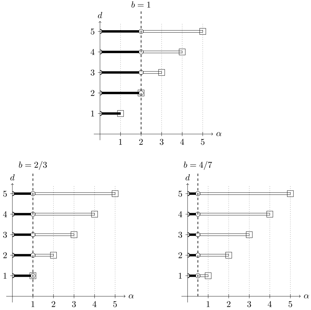
Figure 5: Solvability for the fractional stochastic heat equation in case of a = 2 , b \leq 1 and r = 0 . See Figure 2 for the legends.
