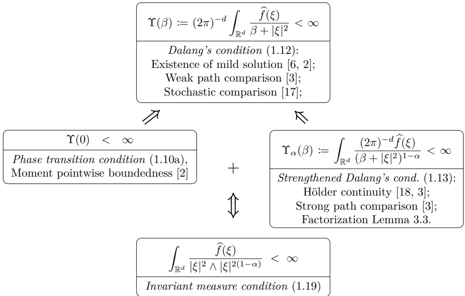
Fig. 1.1 Two conditions—(1.10a) and (1.13)—on \widehat{f} , or equivalent condition (1.19), needed for the main result—Theorem 1.3,
