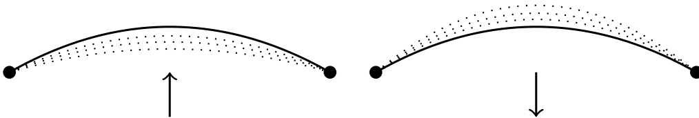
Figure 1.4: A still shot of two vibrating strings at the same position but moving in opposite directions.
