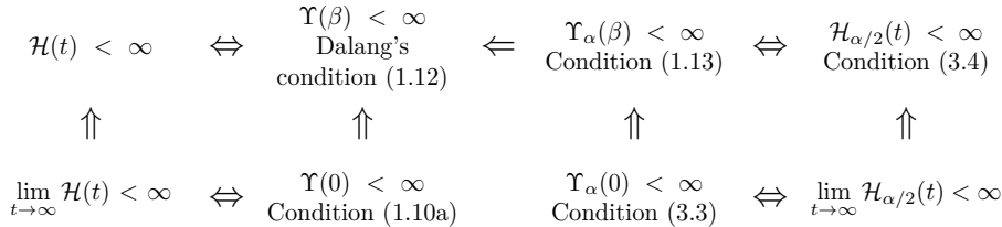
FIG. 2. Relations among various conditions where \alpha \in (0, 1) and \beta > 0 .
