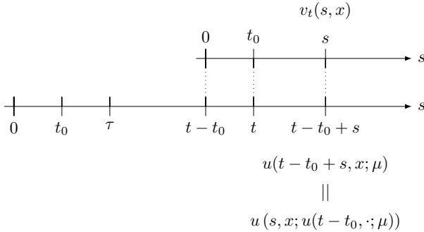
Fig. 4.3 An illustration for the restarted SHE in (4.1).
