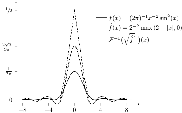
Fig. 5.4 One example that \mathcal{F}^{-1}(\sqrt{\widehat{f}})(x) assumes both positive and negative values.
