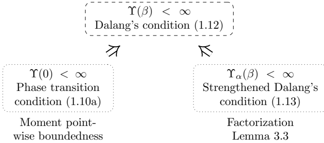
Fig. 1.1 Two conditions—(1.10a) and (1.13)—on \widehat{f} needed for the main result — Theorem 1.3.
