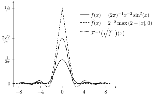
Fig. 5.4 One example that \mathcal{F}^{-1}(\sqrt{\widehat{f}})(x) assumes both positive and negative values.
