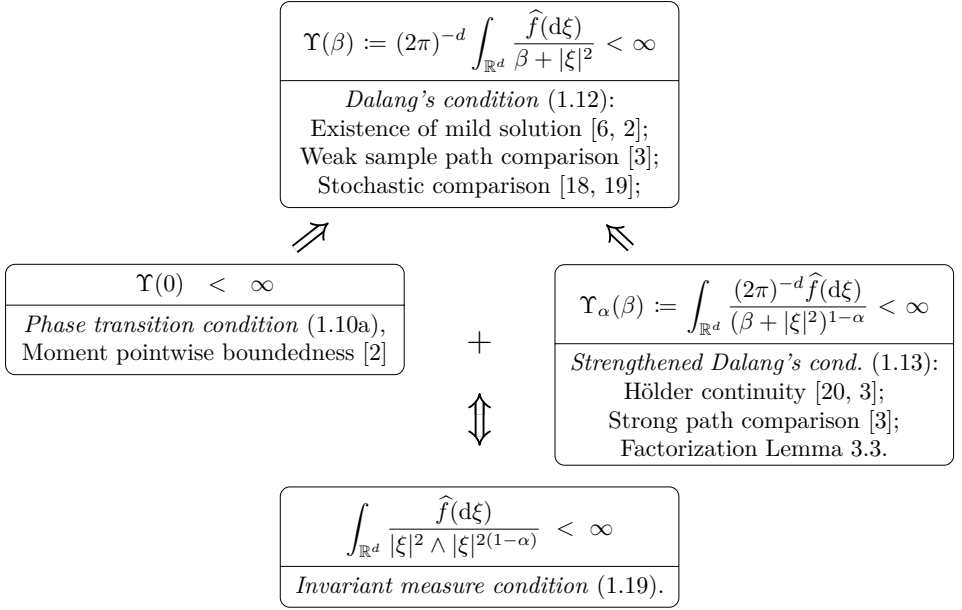
Fig. 1.1 Conditions on the spectral measure \widehat{f} and their implications.
