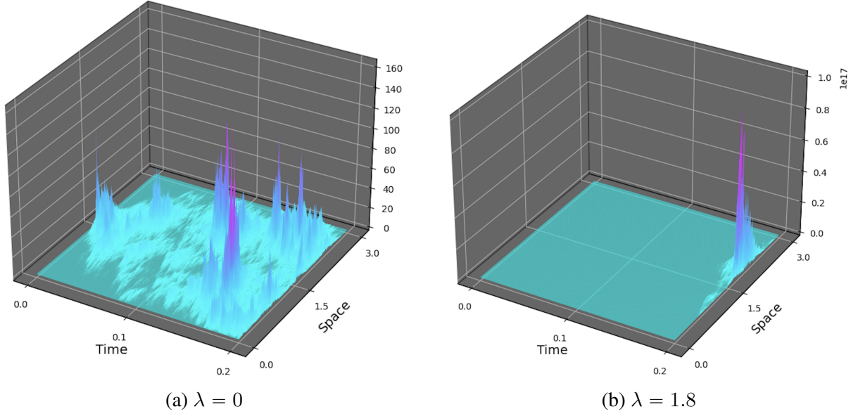
Figure 1.2: Simulations of Equation (1.0.2) with d = 1 , \zeta(\cdot) = \delta_0(\cdot) and b(u) = \lambda u .
