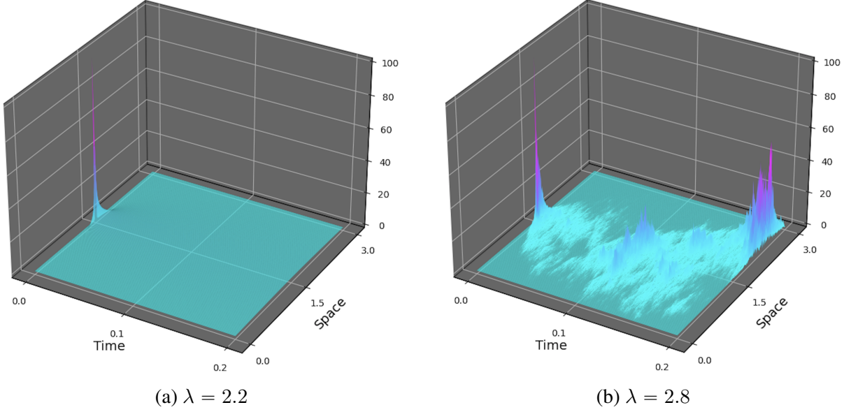
Figure 1.1: Simulations of Equation (1.0.2) with d = 1 , \zeta(\cdot) = \delta_0(\cdot) and b(u) = \lambda u .
