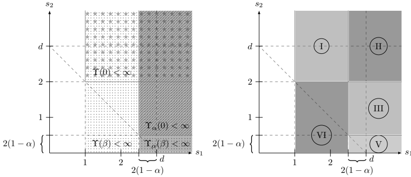
Fig. 5.5 Left figure: Parameter regions for the four conditions: \Upsilon(\beta) < \infty (the dotted region), \Upsilon(0) < \infty (the star-patterned one), \Upsilon_\alpha(0) < \infty (the one with north east lines), and \Upsilon_\alpha(\beta) < \infty (the shaded one). Right figure: five parameter regions that correspond to the relation between (\Upsilon(\beta), \Upsilon(0), \Upsilon_\alpha(\beta), \Upsilon_\alpha(0)) and (\infty, \infty, \infty, \infty) .
