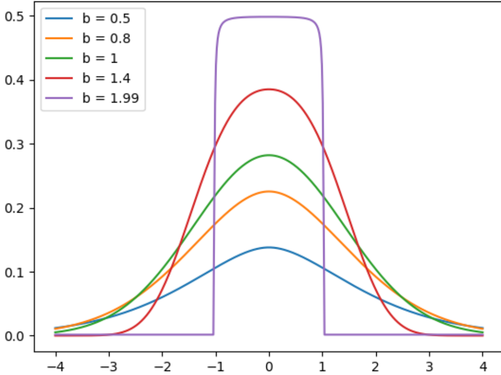
Figure 1.5: Cross sections of G_{2,b,0,2,1}(t, x) with -4 \leq x \leq 4 and t = 1 .
