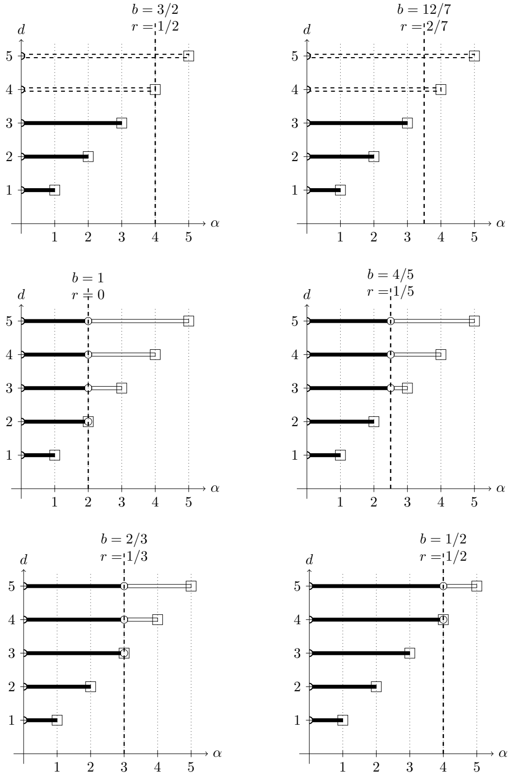
Figure 4: Solvability for the fractional SPDEs in case of a = 2 and r = [b] - b . See Figures 2 and 3 for the legend.
