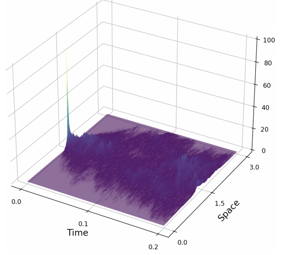
(b) \lambda = 1
