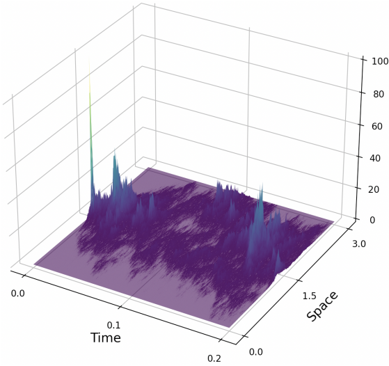
(c) \lambda = 1.8
