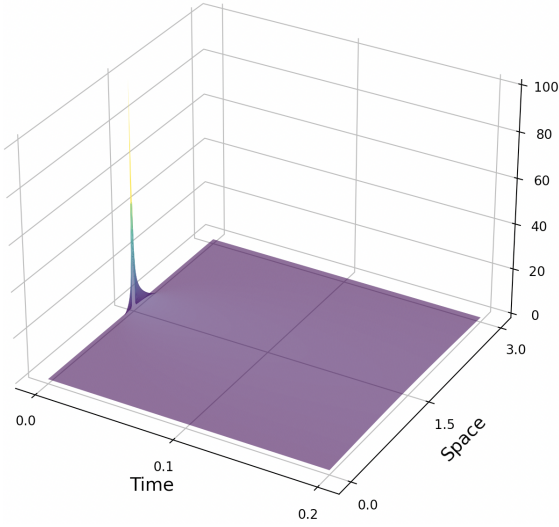
(a) \lambda = 0
