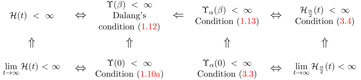
Figure 2: Relations among various conditions where \alpha \in (0, 1) and \beta > 0 .
