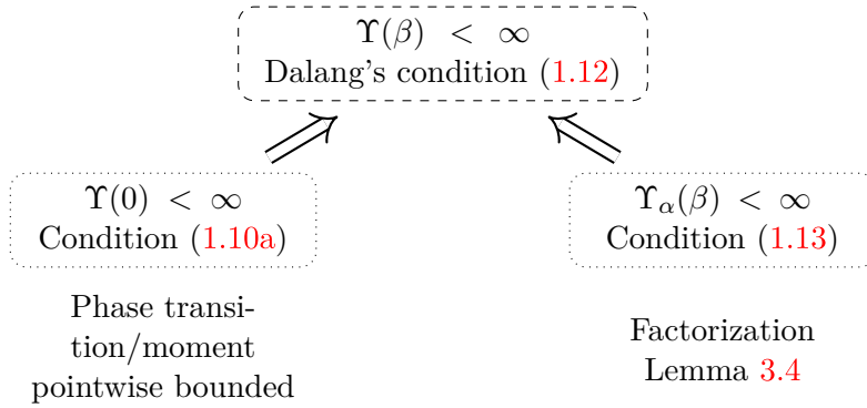
Figure 1: Two conditions—(1.10a) and (1.13)—on \hat{f} needed for the main result — Theorem 1.5.
