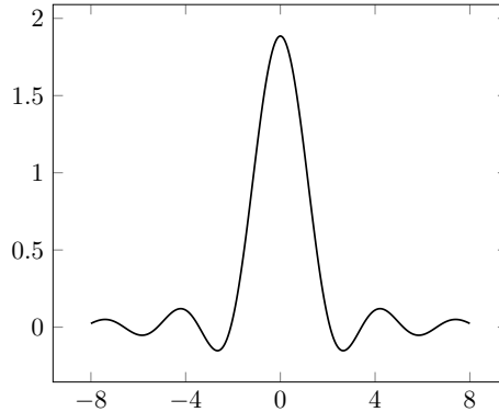
Figure 2: A plot of \mathcal{F}^{-1}\left(\sqrt{\widehat{f}}\right)(x) for \widehat{f}(\xi) = 2^{-2} \max\{2 - |\xi|, 0\} with -8 \leq x \leq 8 .
