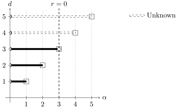
Figure 3: Solvability for the stochastic wave equation (i.e., a = b = 2 and r = 0 ). See Figure 2 for an additional legend.
