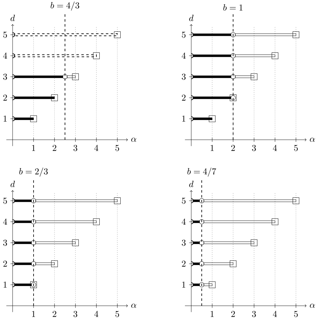
Figure 5: Solvability for the fractional SPDEs in case of a = 2 and r = 0 . See Figures 2 and 3 for the legend.
