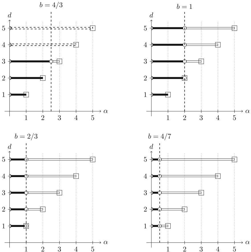
Fig. 5 Solvability for the fractional SPDEs in case of a = 2 and r = 0 . See Figs. 2 and 3 for the legend
