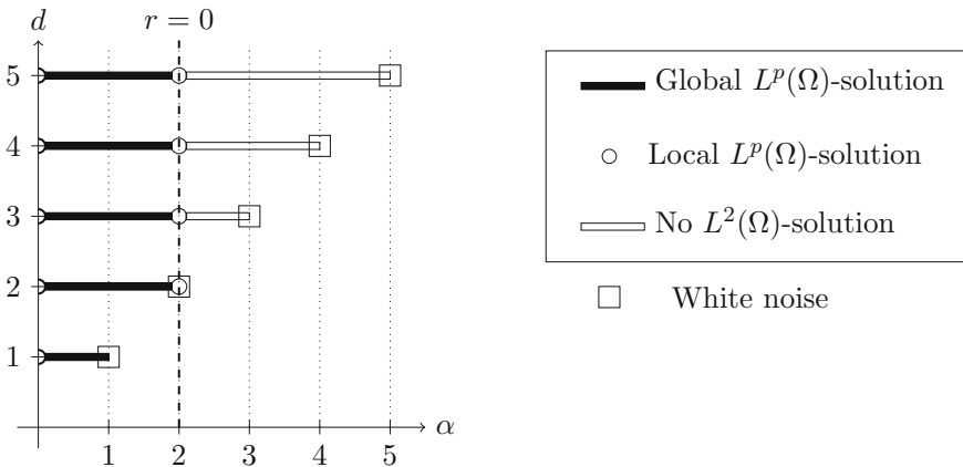
Fig. 2 Solvability for the stochastic heat equation (i.e., a = 2 , b = 1 and r = 0 ) with p \geq 2
