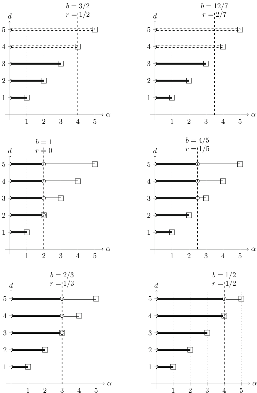
Fig. 4 Solvability for the fractional SPDEs in case of a = 2 and r = [b] - b . See Figs. 2 and 3 for the legend
