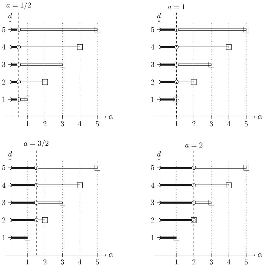
Fig. 6 Solvability for the stochastic heat equation with fractional Laplacian, i.e., the case when b = 1 and r = 0 . See Figs. 2 and 3 for the legend
