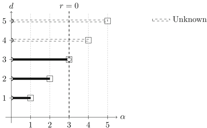
Fig. 3 Solvability for the stochastic wave equation (i.e., a = b = 2 and r = 0 ). See Fig. 2 for an additional legend
