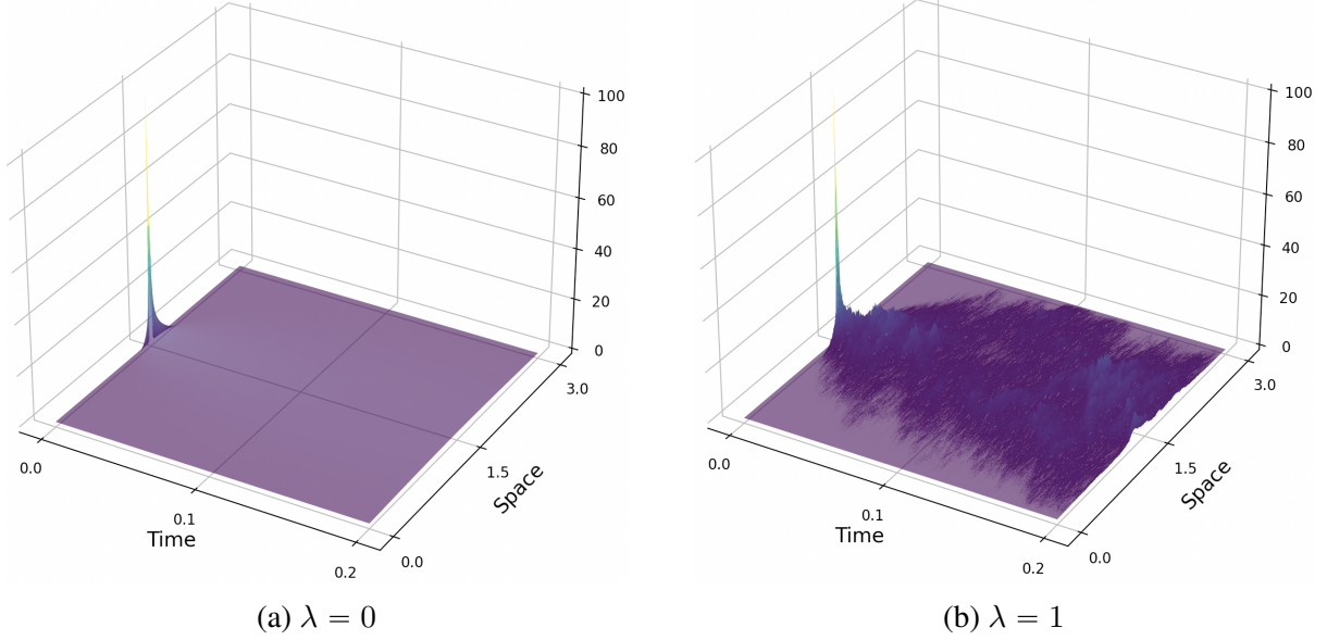
Figure 1.1: Simulations of Equation (1.0.2) with d = 1 , \zeta(\cdot) = \delta_0(\cdot) and b(u) = \lambda u .
