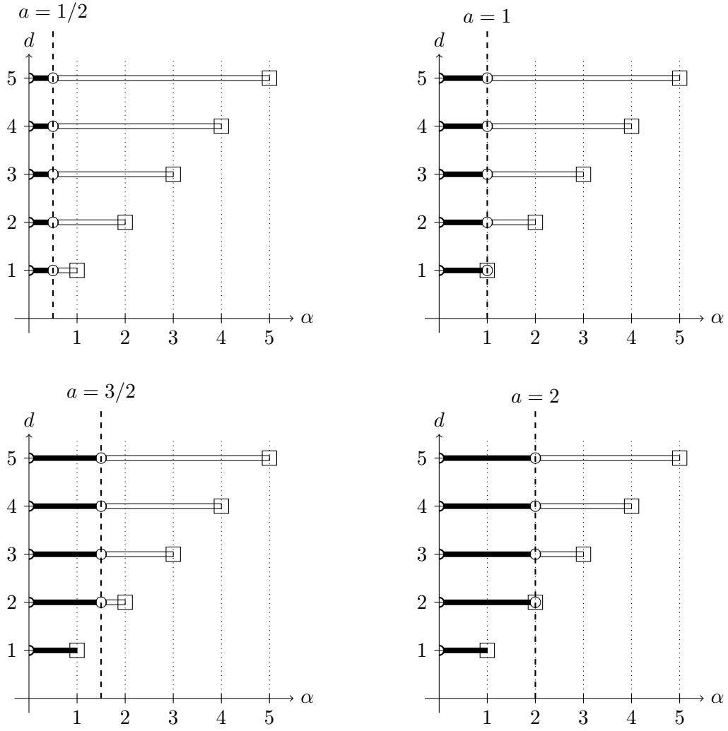
Figure 6: Solvability for the stochastic heat equation with fractional Laplace, i.e, the case when b = 1 and r = 0 . See Figures 2 and 3 for the legend.
