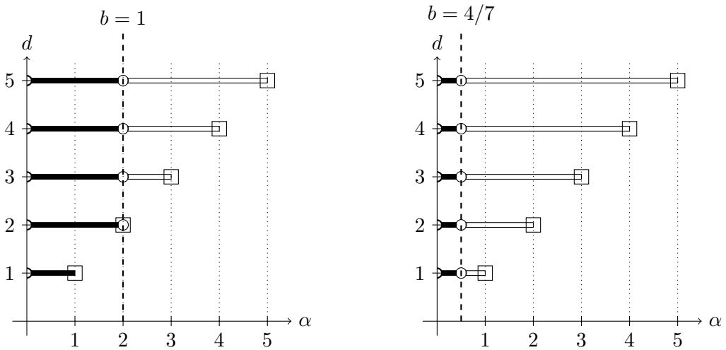
Figure 5: Solvability for the fractional stochastic heat equation in case of a = 2 , b \leq 1 and r = 0 . See Figure 2 for the legends.
