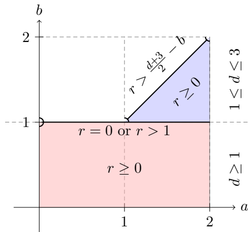
Figure 1: Illustration of the sufficient conditions (Remark 1.9) for G(t, \cdot) to be nonnegative.
