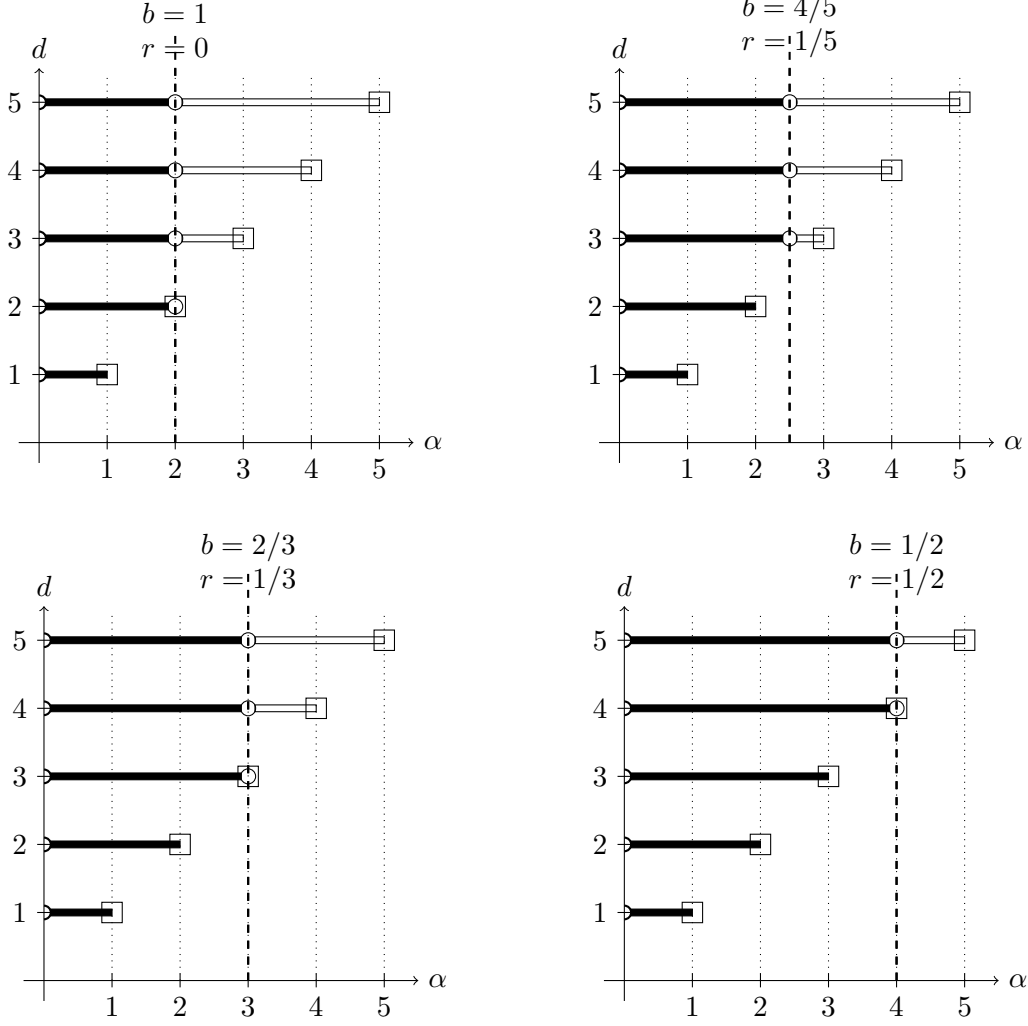
Figure 4: Solvability for the fractional stochastic heat equation in case of a = 2 , b \leq 1 and r = 1 - b . See Figure 2 for the legends.
