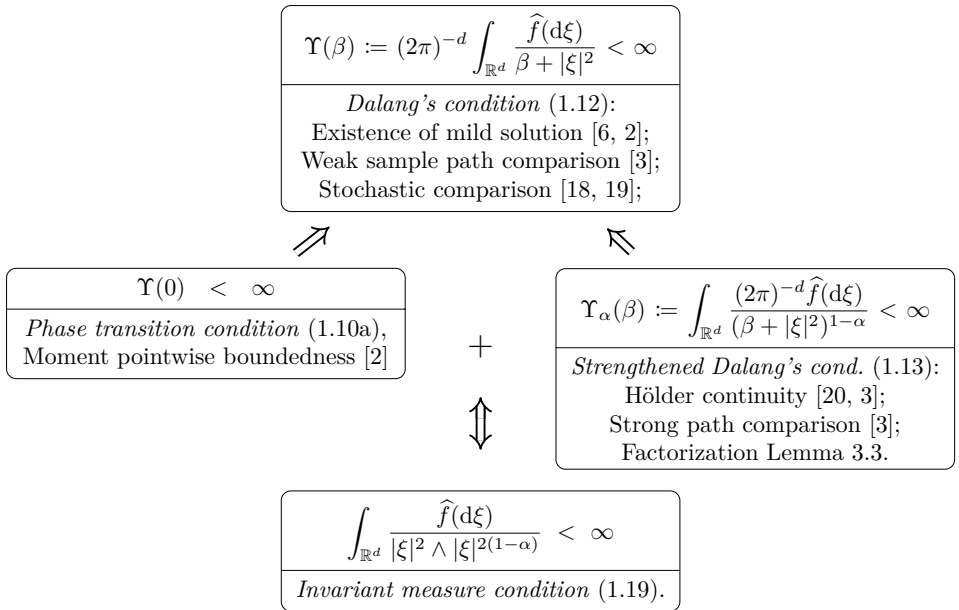
Fig. 1.1 Conditions on the spectral measure \hat{f} and their implications.
