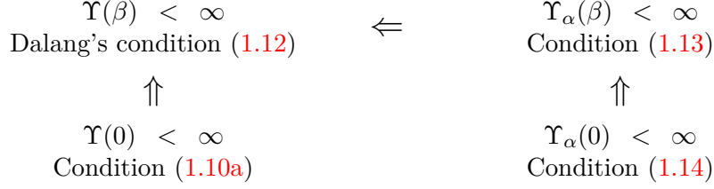
Figure 1: Relations among conditions (1.12), (1.13), (1.14) and (1.10a).
