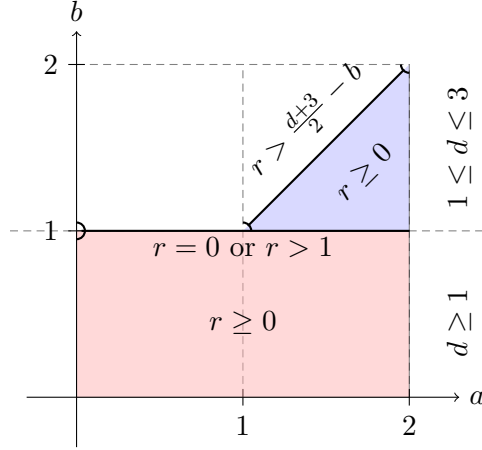
Figure 1: Illustration of the sufficient conditions (Assumption 1.4) for G(t, \cdot) to be nonnegative.
