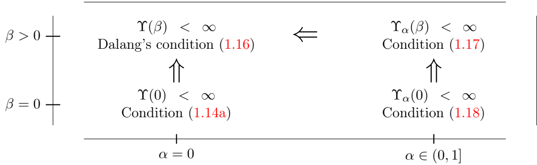
Figure 1: Relations among conditions (1.16), (1.17), (1.18) and (1.14a). Check also Lemma 4.5 for the relation between \Upsilon(0) < \infty and \Upsilon_\alpha(0) < \infty .
