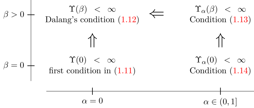
Figure 1: Relations among conditions (1.12), (1.13), (1.14) and the first condition in (1.11). Check also Lemma 4.5 for the relation between \Upsilon(0) < \infty and \Upsilon_\alpha(0) < \infty .
