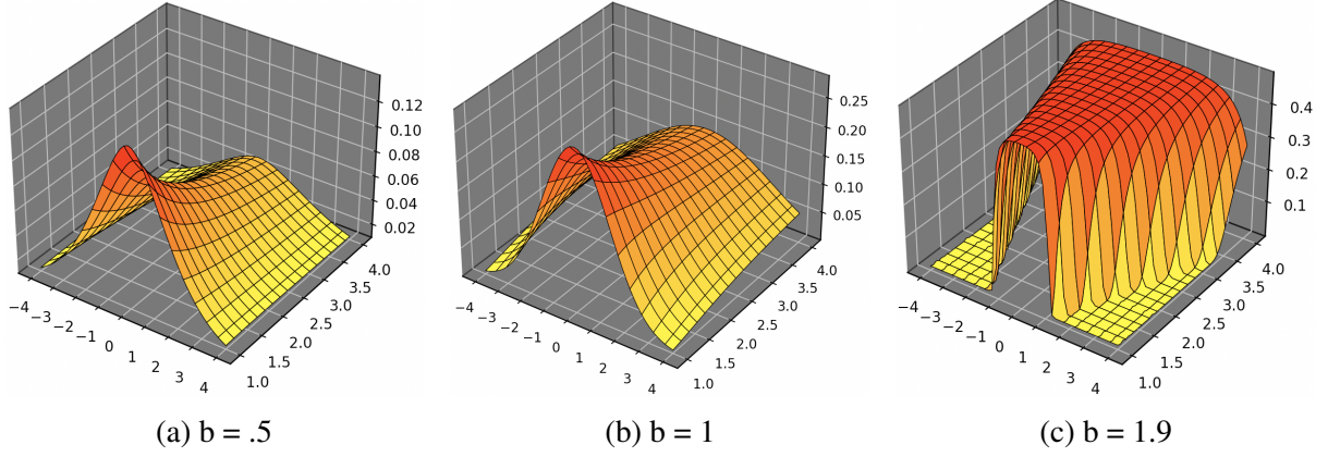
Figure 1.3: Some plots of G_{2,b,0,2,1}(t, x) with -4 \leq x \leq 4 and 1 \leq t \leq 4 .
