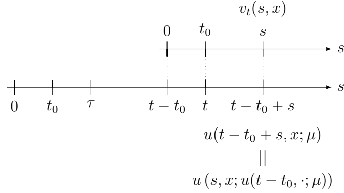
Figure 3.3: An illustration for the restarted SHE in (3.5.1).
