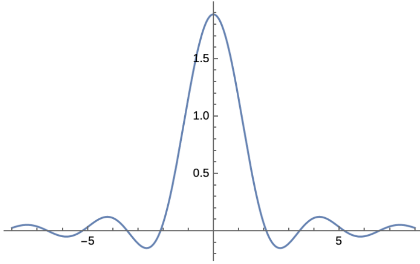
Figure 3.2: A plot of \mathcal{F}^{-1} \left( \sqrt{\hat{f}} \right) (\zeta) for \hat{f}(\xi) = 2^{-2} \max\{2 - |\xi|, 0\} with -8 \leq \zeta \leq 8 .
