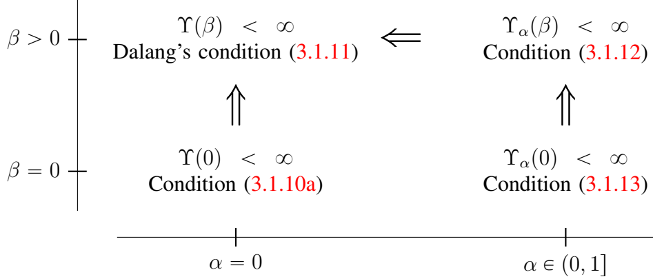
Figure 3.1: Relations among conditions (3.1.11), (3.1.12), (3.1.13) and (3.1.10a). Check also Lemma 3.4.5 for the relation between \Upsilon(0) < \infty and \Upsilon_\alpha(0) < \infty .
