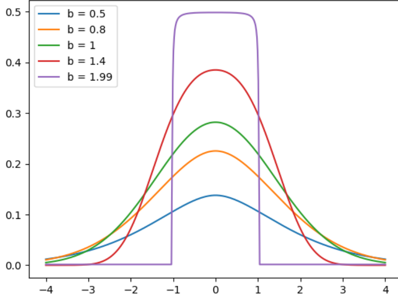
Figure 1.4: Cross sections of G_{2,b,0,2,1}(t, x) with -4 \leq x \leq 4 and t = 1 .
