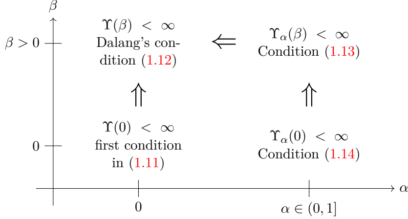
Figure 1: Relations among conditions (1.12), (1.13), (1.14) and the first condition in (1.11). Check also Lemma 4.5 for the relation between \Upsilon(0) < \infty and \Upsilon_\alpha(0) < \infty .
