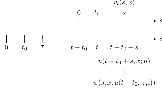
Figure 2: Some illustrations for the restarted SHE in (5.1).
