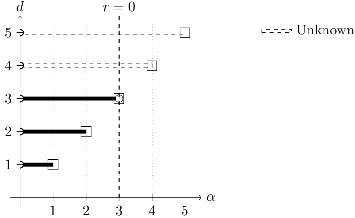
Figure 3: Solvability for the stochastic wave equation (i.e., a = b = 2 and r = 0 ). See Figure 2 for more legends.
