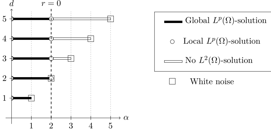
Figure 2: Solvability for the stochastic heat equation (i.e., a = 2 , b = 1 and r = 0 ) with p \geq 2 .
