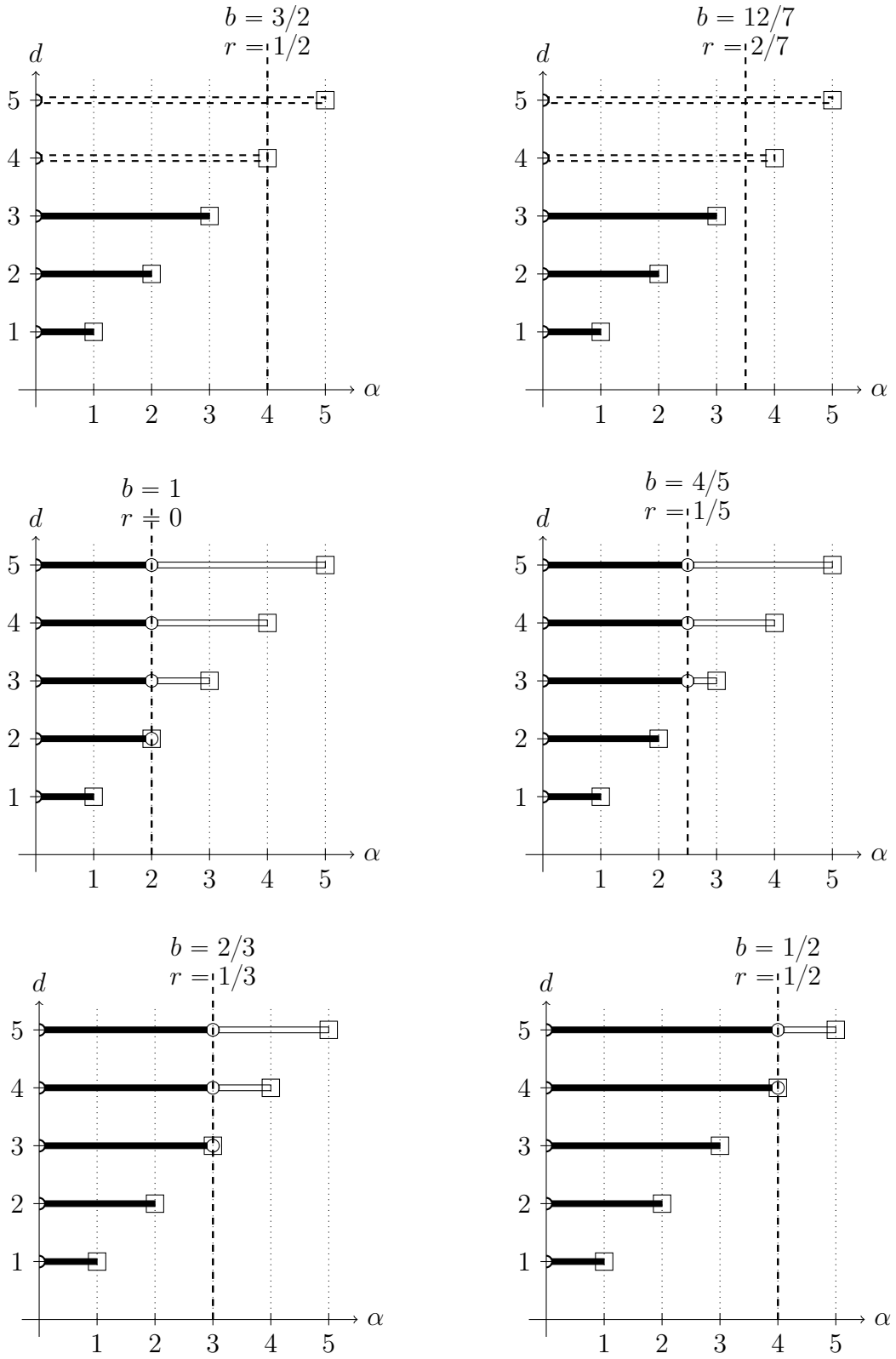
Figure 3.4: Solvability for the fractional SPDEs in case of a = 2 and r = [b] - b . See Figures 3.2 and 3.3 for the legend.
