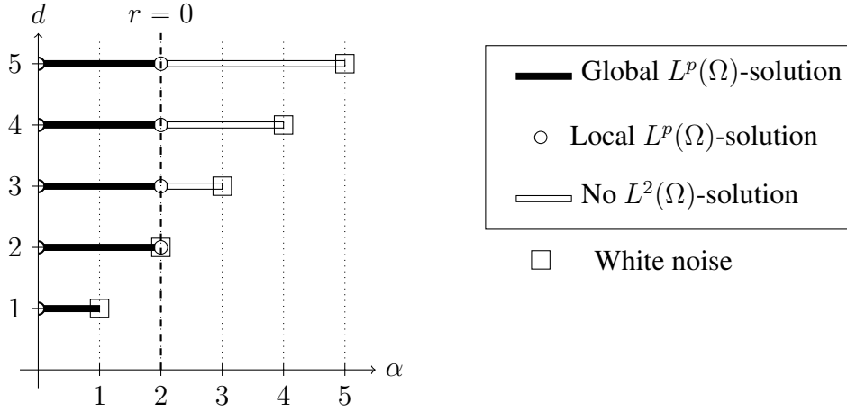
Figure 3.2: Solvability for the stochastic heat equation (i.e., a = 2 , b = 1 and r = 0 ) with p \geq 2 .
