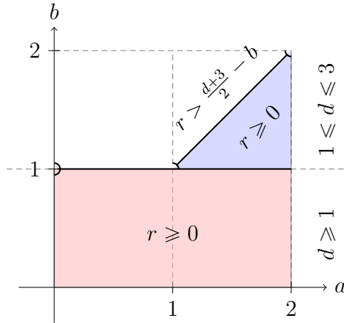
Figure 3.1: Illustration of the sufficient conditions (Remark 3.1.2) for G(t, \cdot) to be nonnegative.
