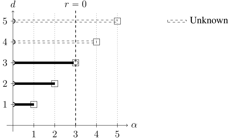
Figure 3.3: Solvability for the stochastic wave equation (i.e., a = b = 2 and r = 0 ). See Figure 3.2 for an additional legend.
