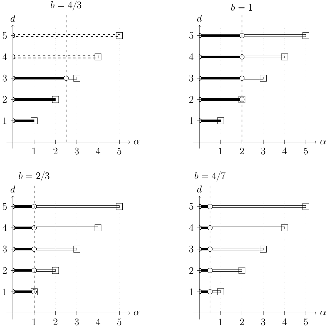
Figure 3.5: Solvability for the fractional SPDEs in case of a = 2 and r = 0 . See Figures 3.2 and 3.3 for the legend.
