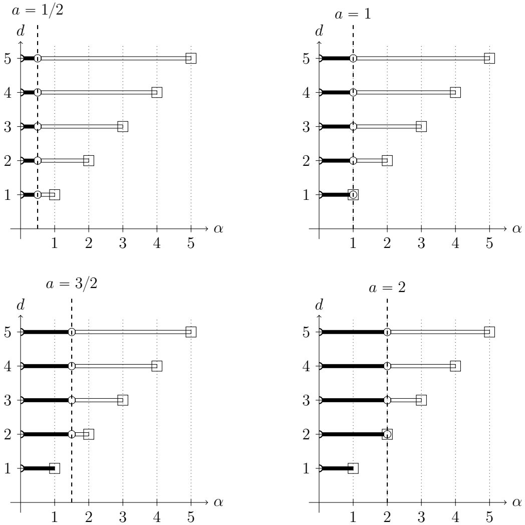
Figure 3.6: Solvability for the stochastic heat equation with fractional Laplacian, i.e, the case when b = 1 and r = 0 . See Figures 3.2 and 3.3 for the legend.
