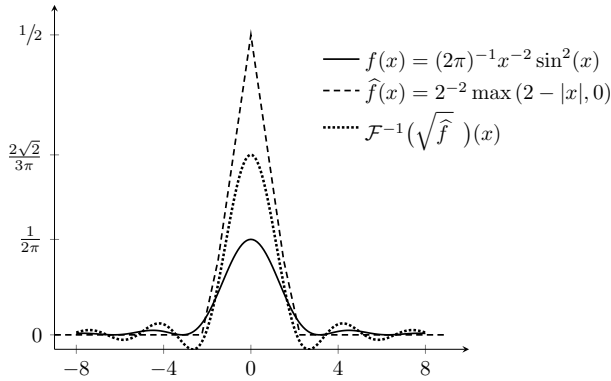
Fig. 5.4 One example that \mathcal{F}^{-1}(\sqrt{\hat{f}})(x) assumes both positive and negative values.
