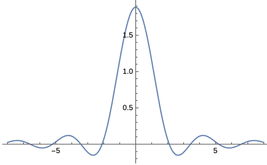
Figure 2: A plot of \mathcal{F}^{-1} \left( \sqrt{\hat{f}} \right) (x) for \hat{f}(\xi) = 2^{-2} \max\{2 - |\xi|, 0\} with -8 \leq x \leq 8 .
