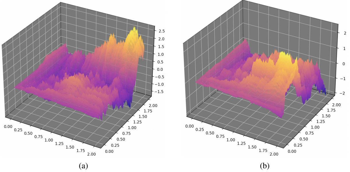
Figure 1.3: A simulation of two sample paths of a Brownian sheet.
