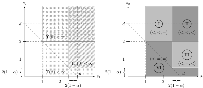
Fig. 5.5 Left figure: Parameter regions for the three conditions: \Upsilon(\beta) < \infty (the dotted region), \Upsilon(0) < \infty (the star-patterned one) and \Upsilon_\alpha(0) < \infty (the one with north east lines). Right figure: four parameter regions that correspond to the relation between (\Upsilon(\beta), \Upsilon(0), \Upsilon_\alpha(0)) and (\infty, \infty, \infty) .
