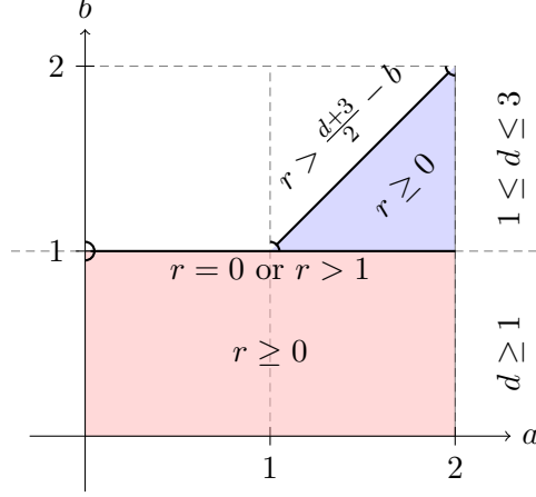
Figure 1: Illustration of the sufficient conditions (Remark 1.8) for G(t, \cdot) to be nonnegative.
