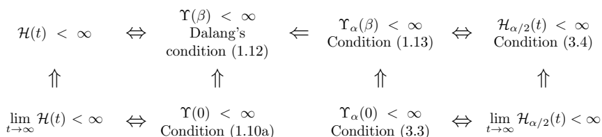
Fig. 3.2 Relations among various conditions where \alpha \in (0, 1) and \beta > 0 .
