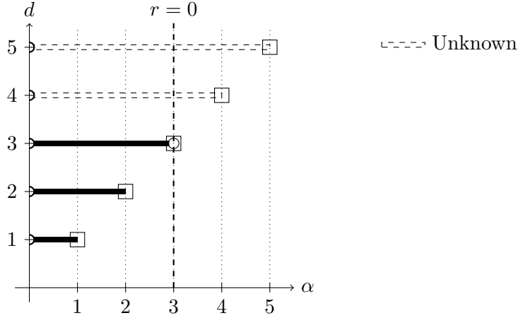
Figure 3: Solvability for the stochastic wave equation (i.e., a = b = 2 and r = 0 ). See Figure 2 for more legends. (F:SWE)
