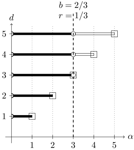
Figure 4: Solvability for the fractional stochastic heat equation in case of a = 2 , b \leq 1 and r = 1 - b . See Figure 2 for the legends.
