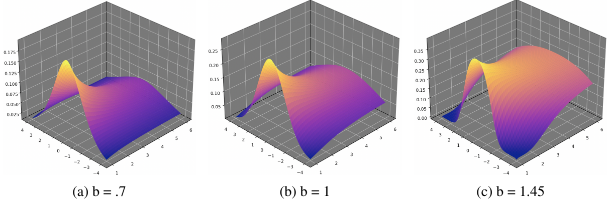
Figure 1.4: Some plots of G_{2,b,0,2,1}(t, x) with -4 \leq x \leq 4 and 1 \leq t \leq 6 .
