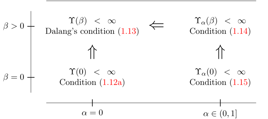
Figure 1: Relations among conditions (1.13), (1.14), (1.15) and (1.12a). Check also Lemma 4.5 for the relation between \Upsilon(0) < \infty and \Upsilon_\alpha(0) < \infty .
